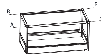
7. Use screws A to screw and fix the corners of the front panel, and screws B for the corners of the rear panel
