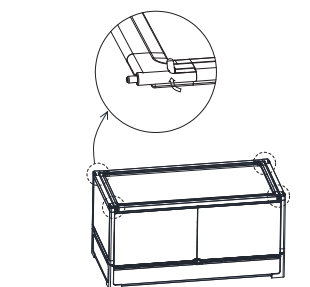
11. Secure the top mesh by closing the tabs at the corners as shown in the image
